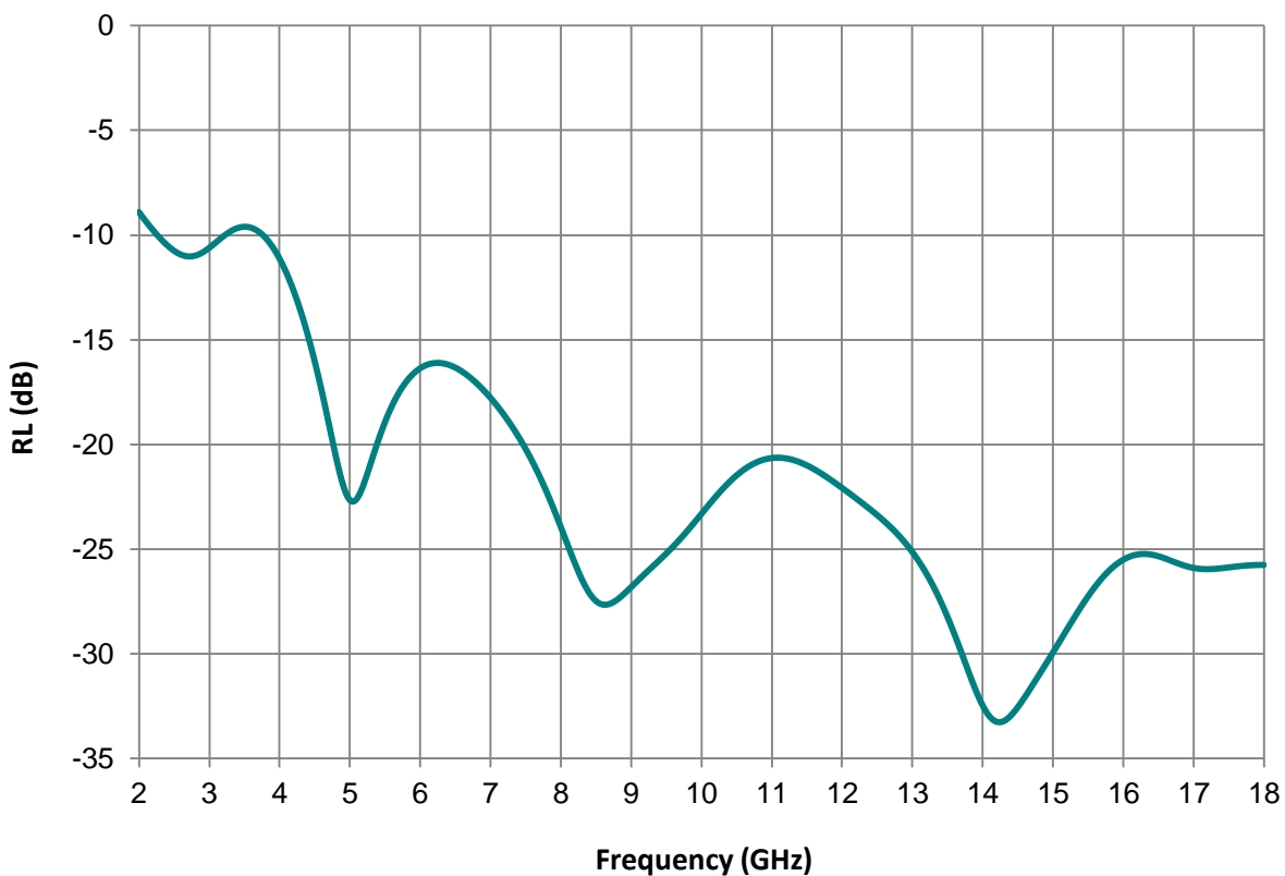
Reflection Loss of RT-10362
