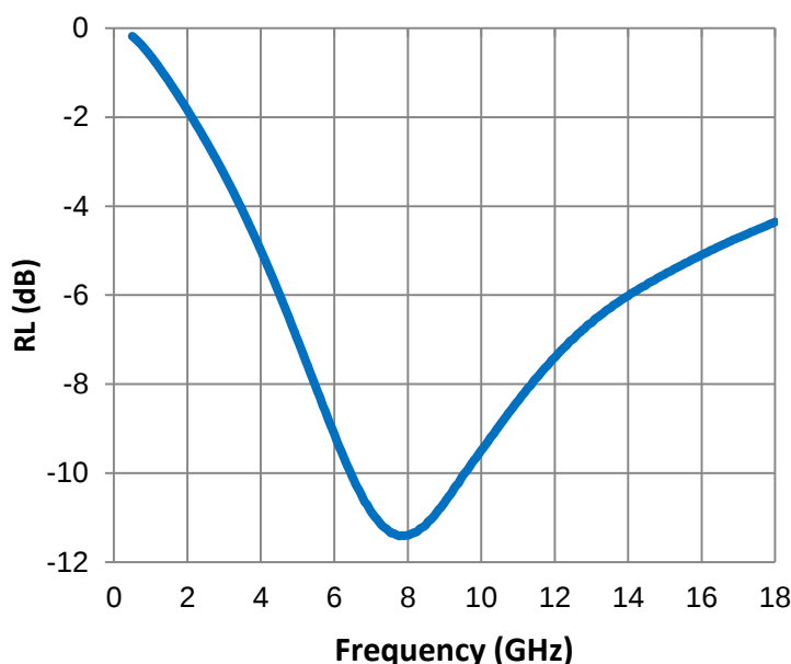
Reflection Loss
