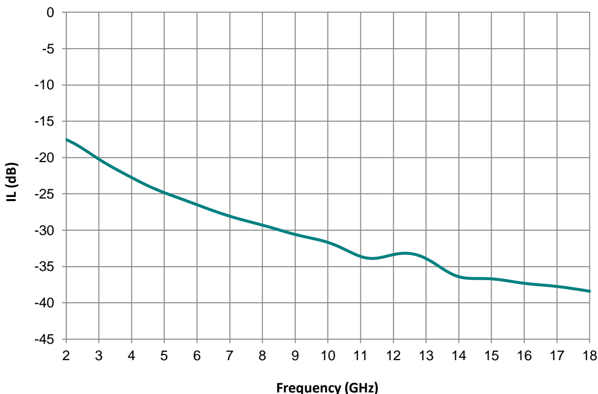
Insertion Loss of LS-55219
